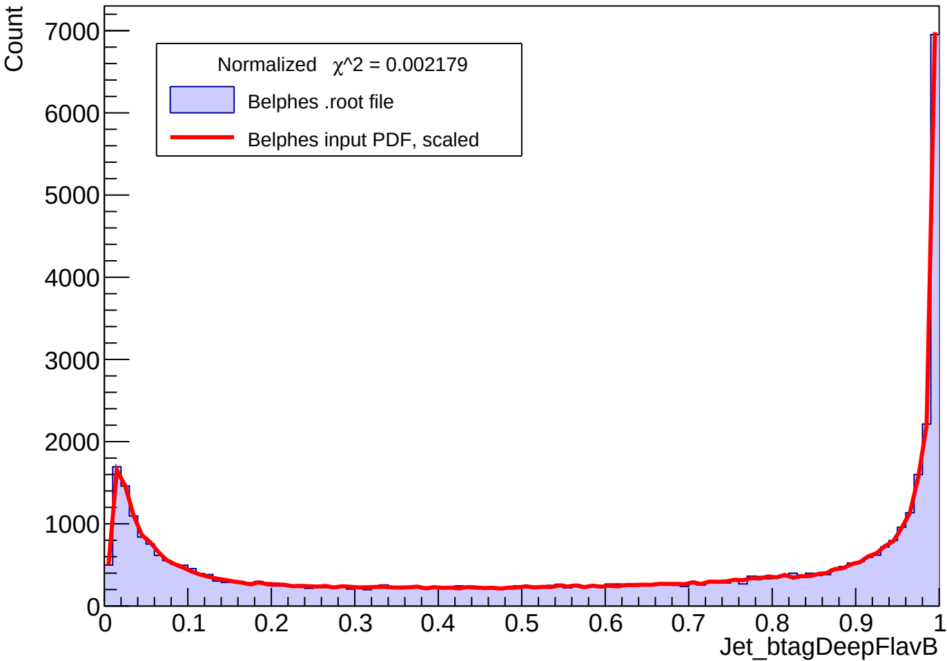
Jet_btagDeepFlavB on PT={20.0, 30.0}, abs(Eta)={0.0, 0.5}
